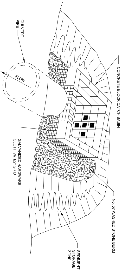
PERSPECTIVE VIEW
