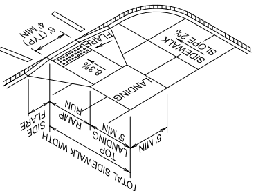
TYPE N-3A
